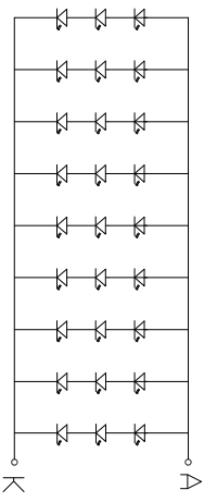
LED CIRCUIT DIAGRAM:
